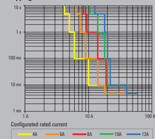
Tripping characteristic normal
