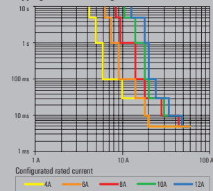
Tripping characteristic lag
